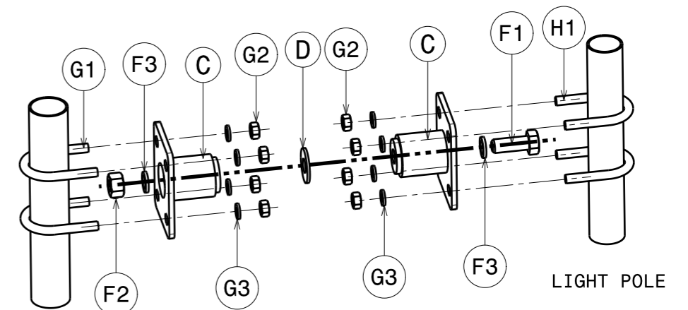
STANCHION
